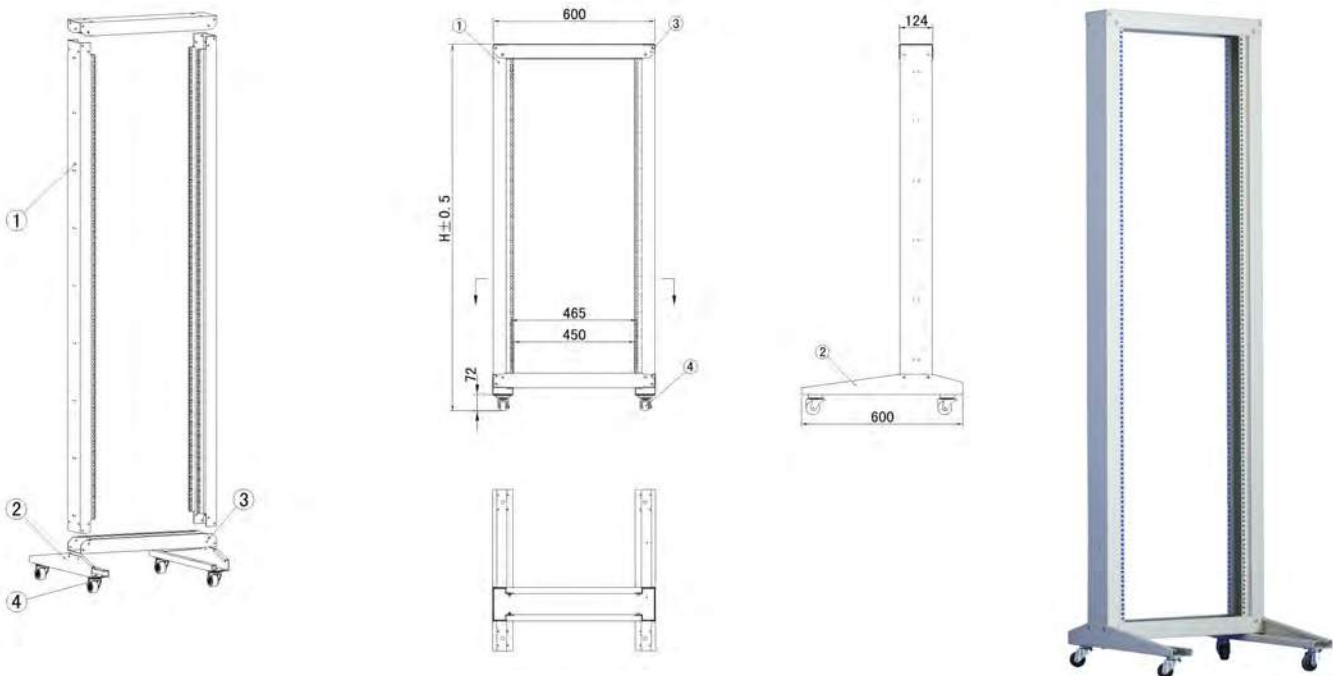
Two post 42U
