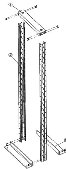
1. Horizontal beam 2. Pole 3. Plinth
