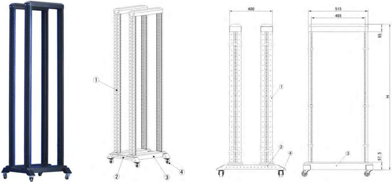
Two post 42U
